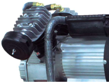
Cabezal dos cilindros y enfriador Two cylinder head and cooler
